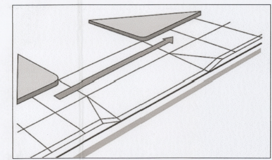
RAMP DETAIL
